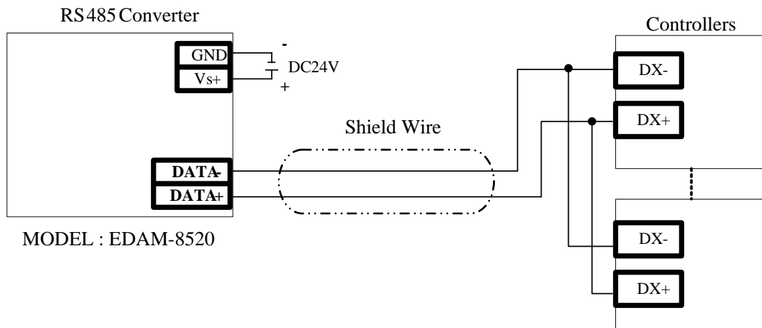
Figure: 3.1-2
